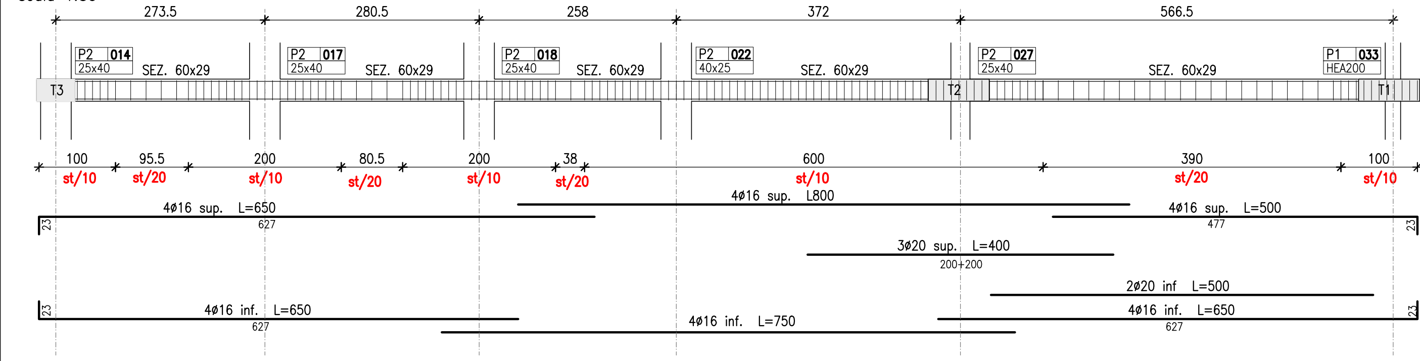
TRAVE T11 scala 1:50
