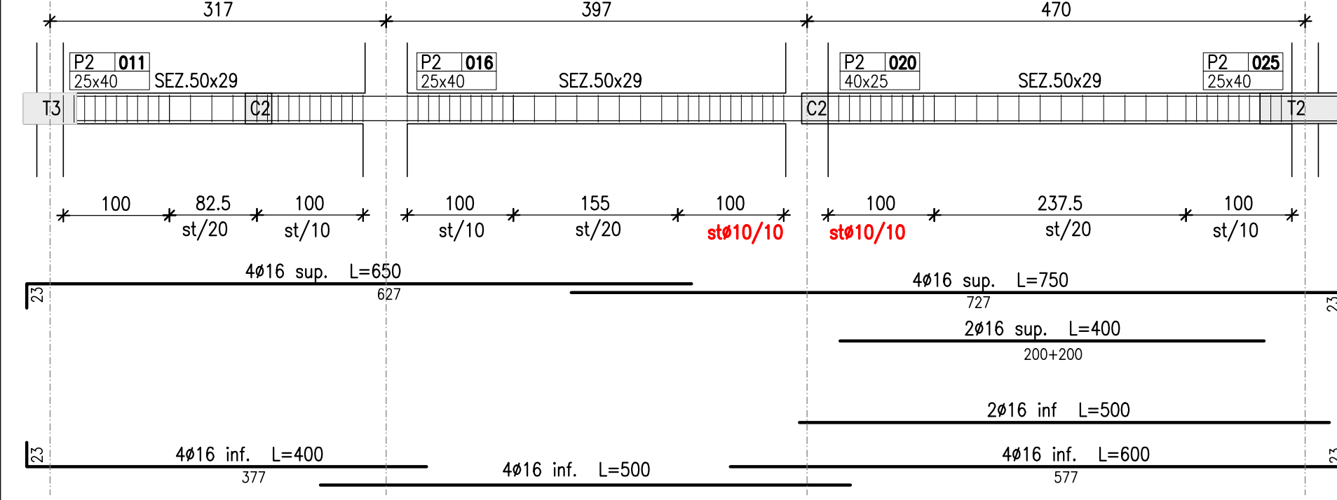
TRAVE T11 scala 1:50
